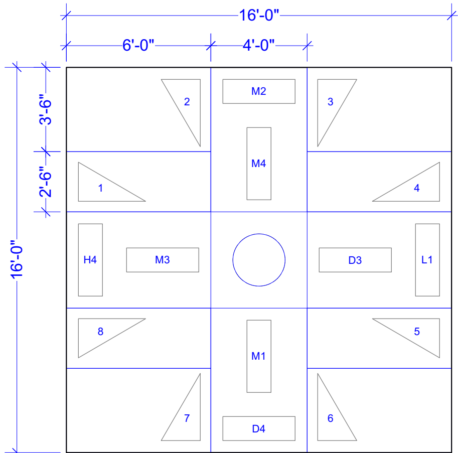
1 PLATFORM LAYOUT & PLEXI LABELS Scale: 1/4" = 1'-0"
