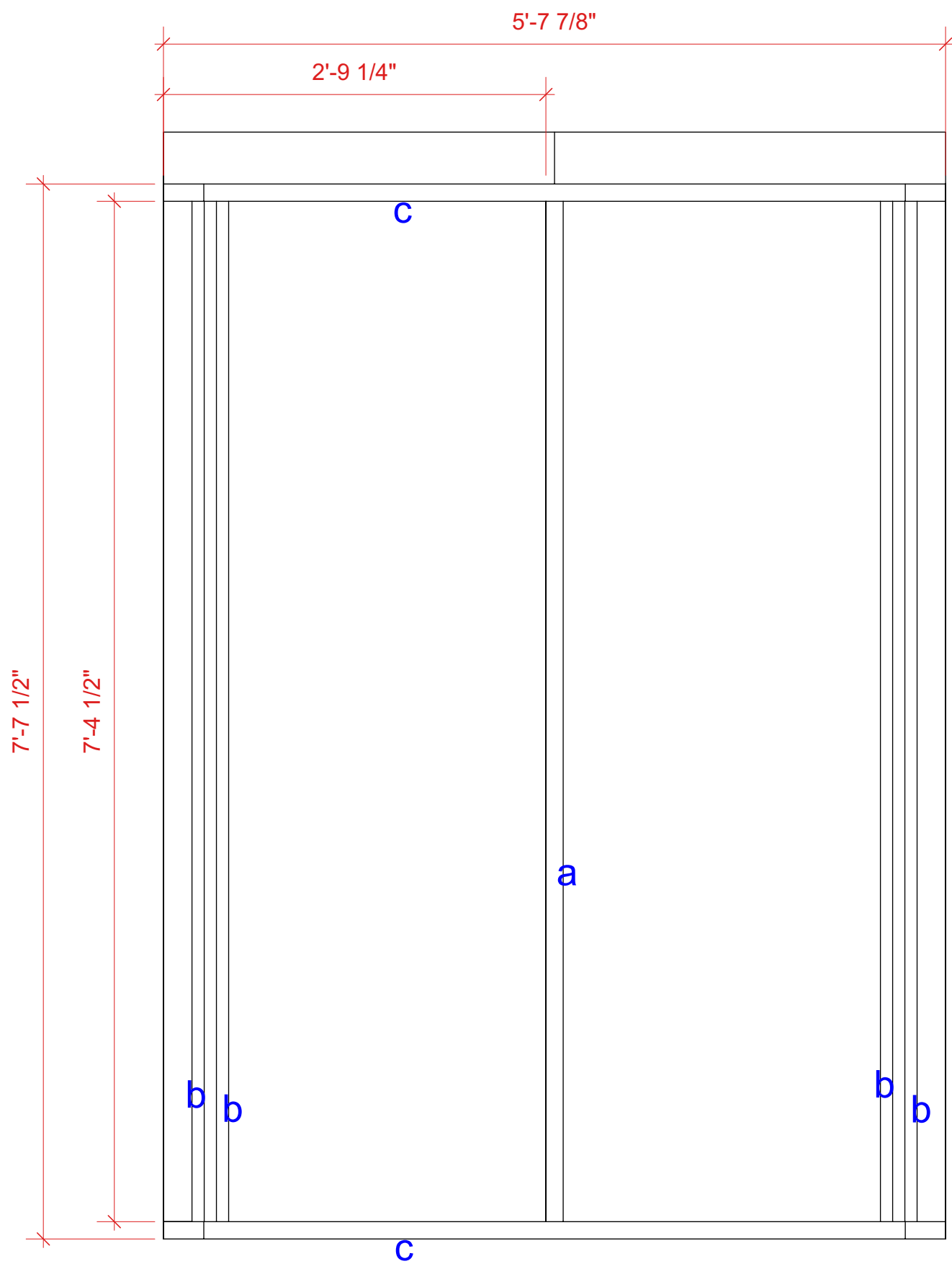
2 FIRST LEVEL WALL C Scale: 1" = 1'-0"
