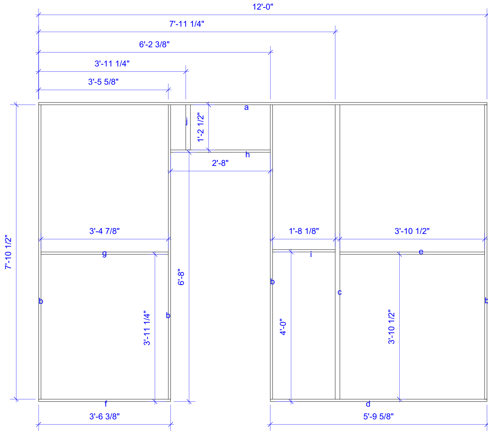
2 SECOND LEVEL BACK WALL B Scale: 3/4" = 1'-0"
