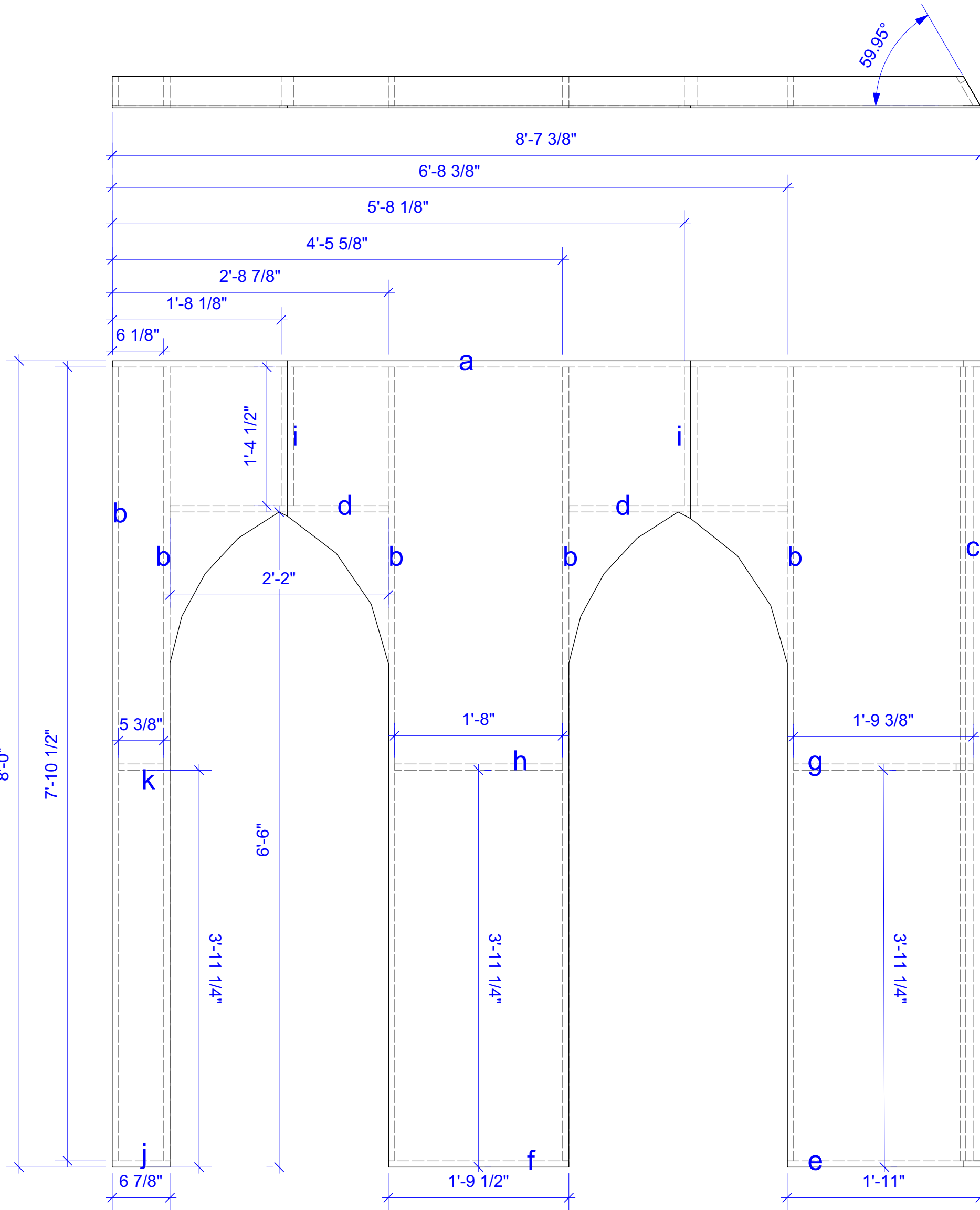
2 SECOND LEVEL FRONT WALL B Scale: 1" = 1'-0"
