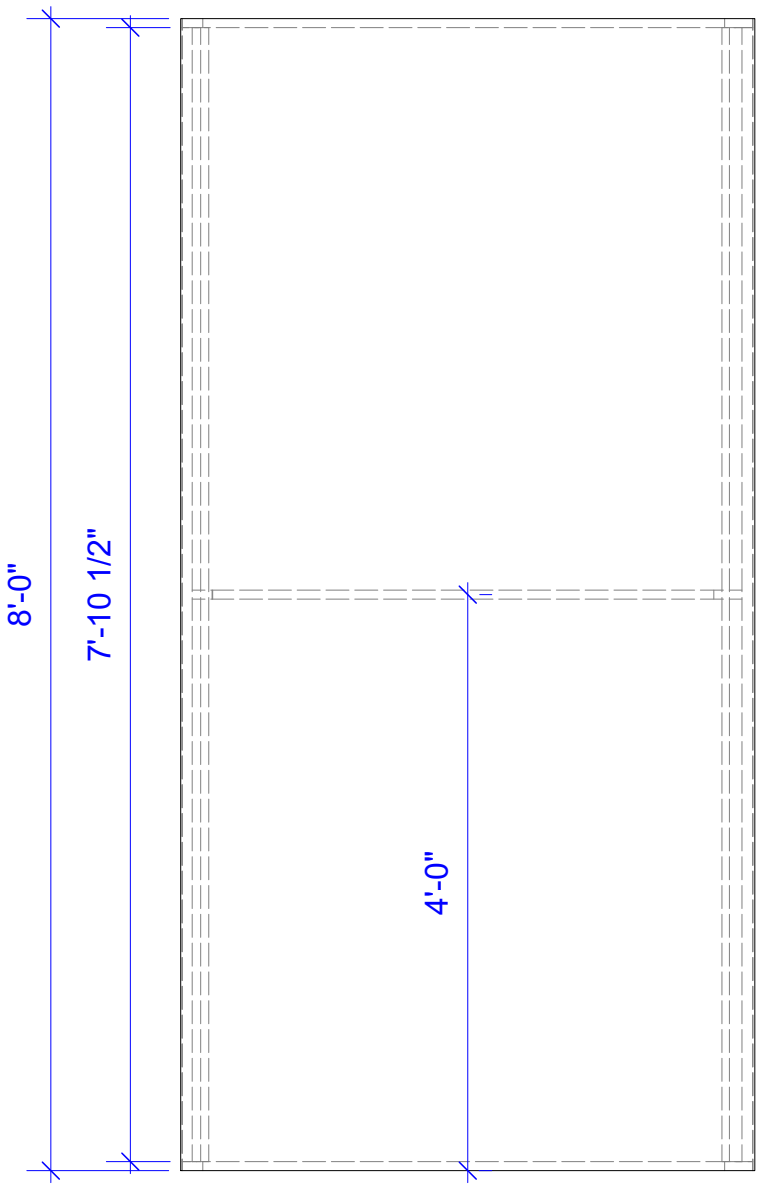
1 SECOND LEVEL ANGLE WALL D Scale: 3/4" = 1'-0"
