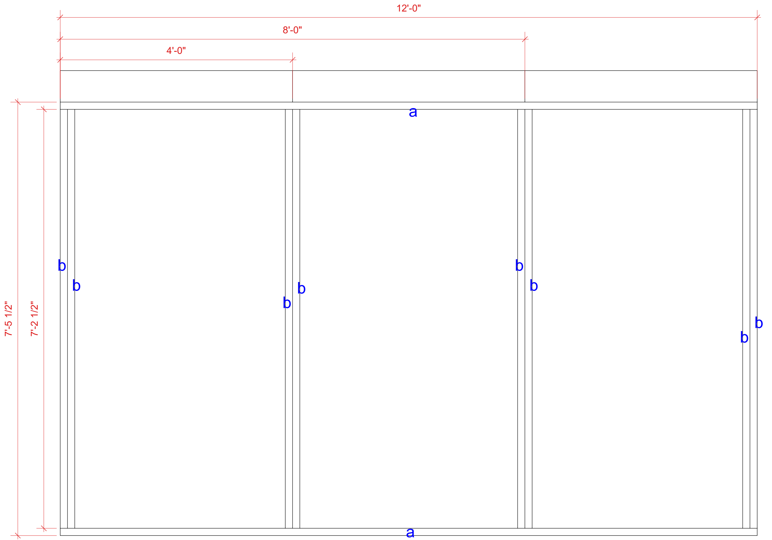
3 FIRST LEVEL WALL D Scale: 1" = 1'-0"
