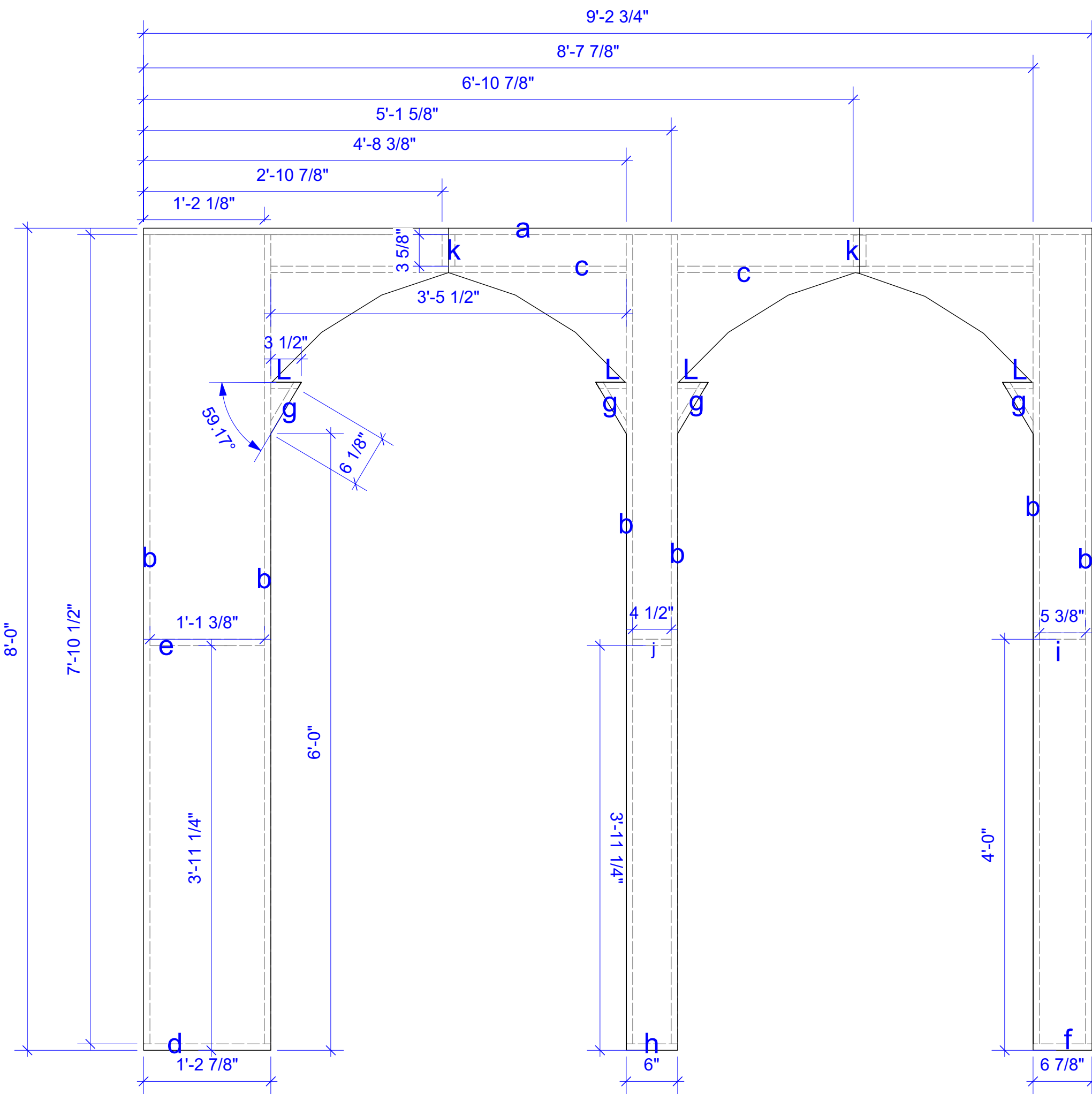
1 SECOND LEVEL FRONT WALL A Scale: 1" = 1'-0"
