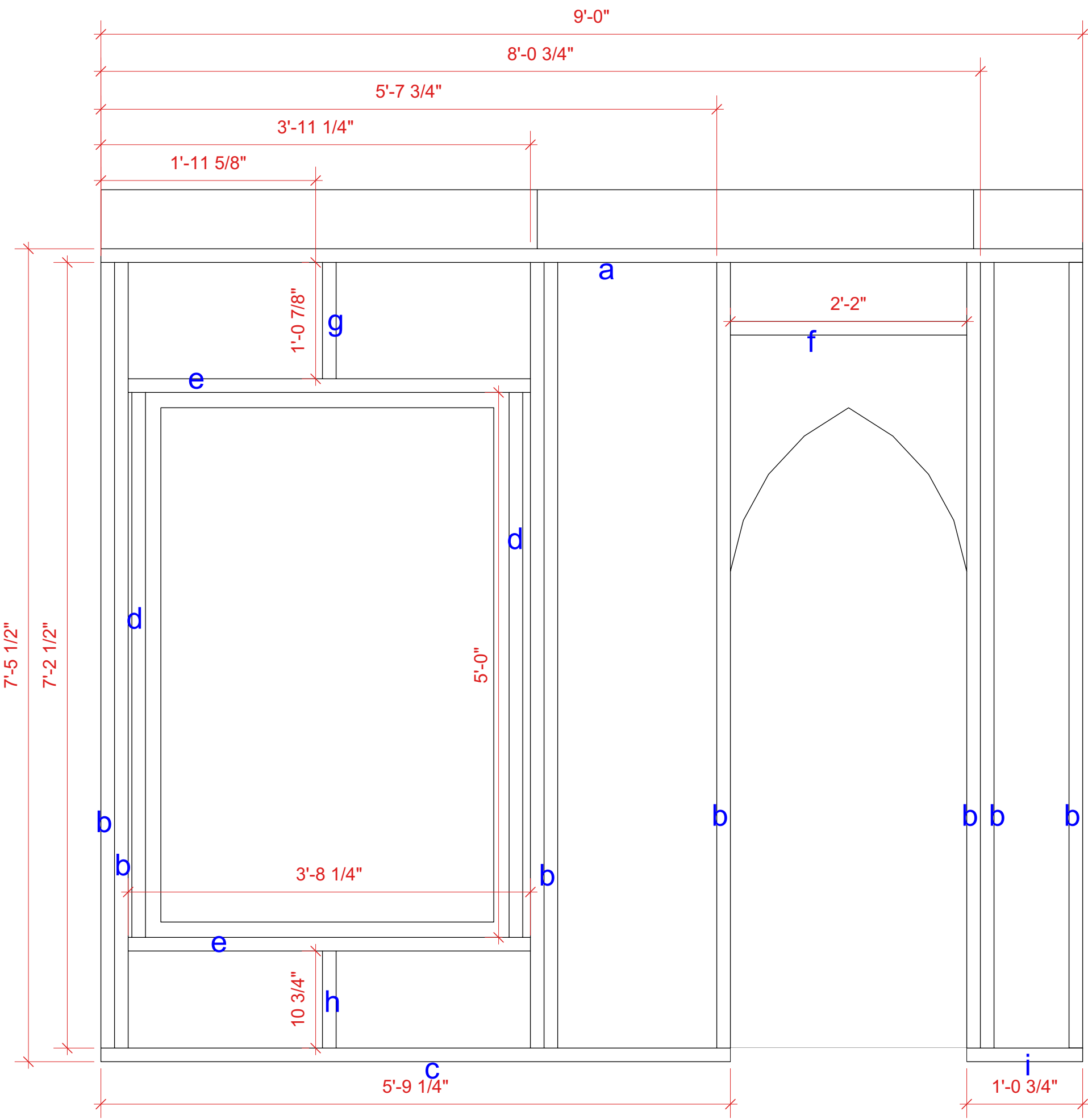
1 FIRST LEVEL WALL B Scale: 1" = 1'-0"
