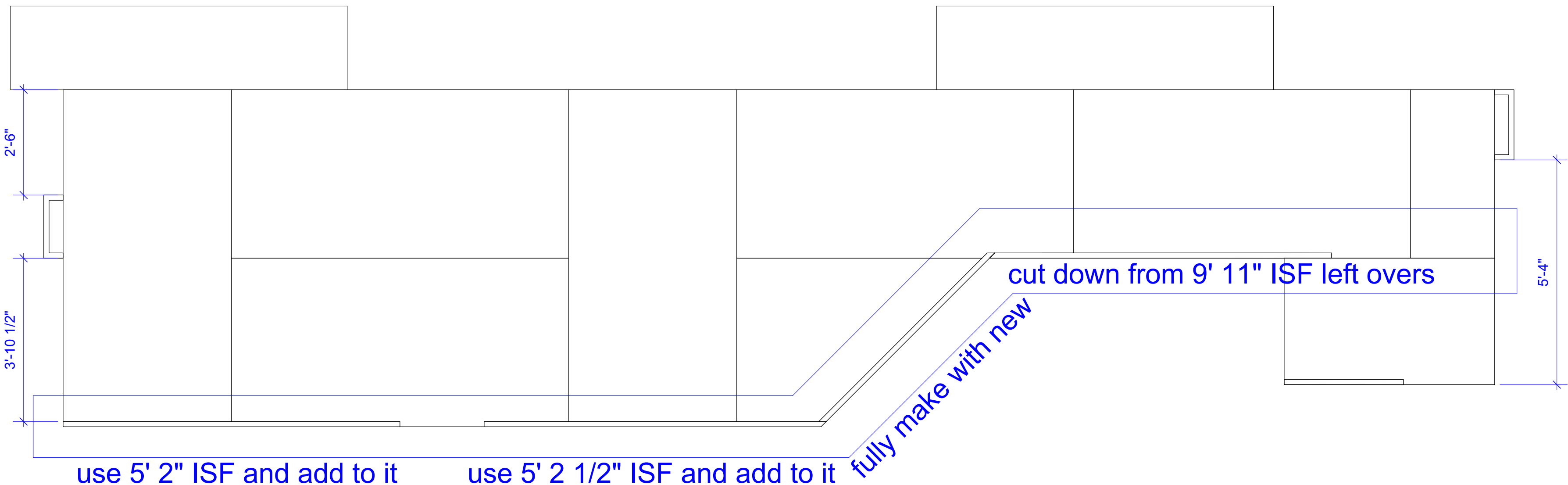
1 GROUND PLAN Scale: 1/2" = 1'-0"
