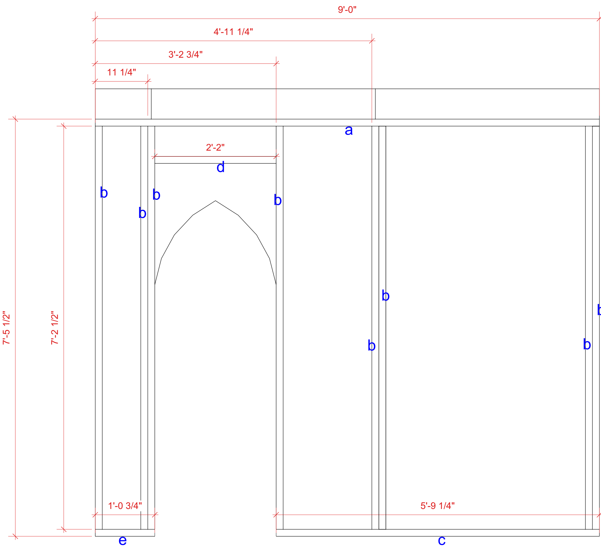
4 FIRST LEVEL WALL A Scale: 1" = 1'-0"
