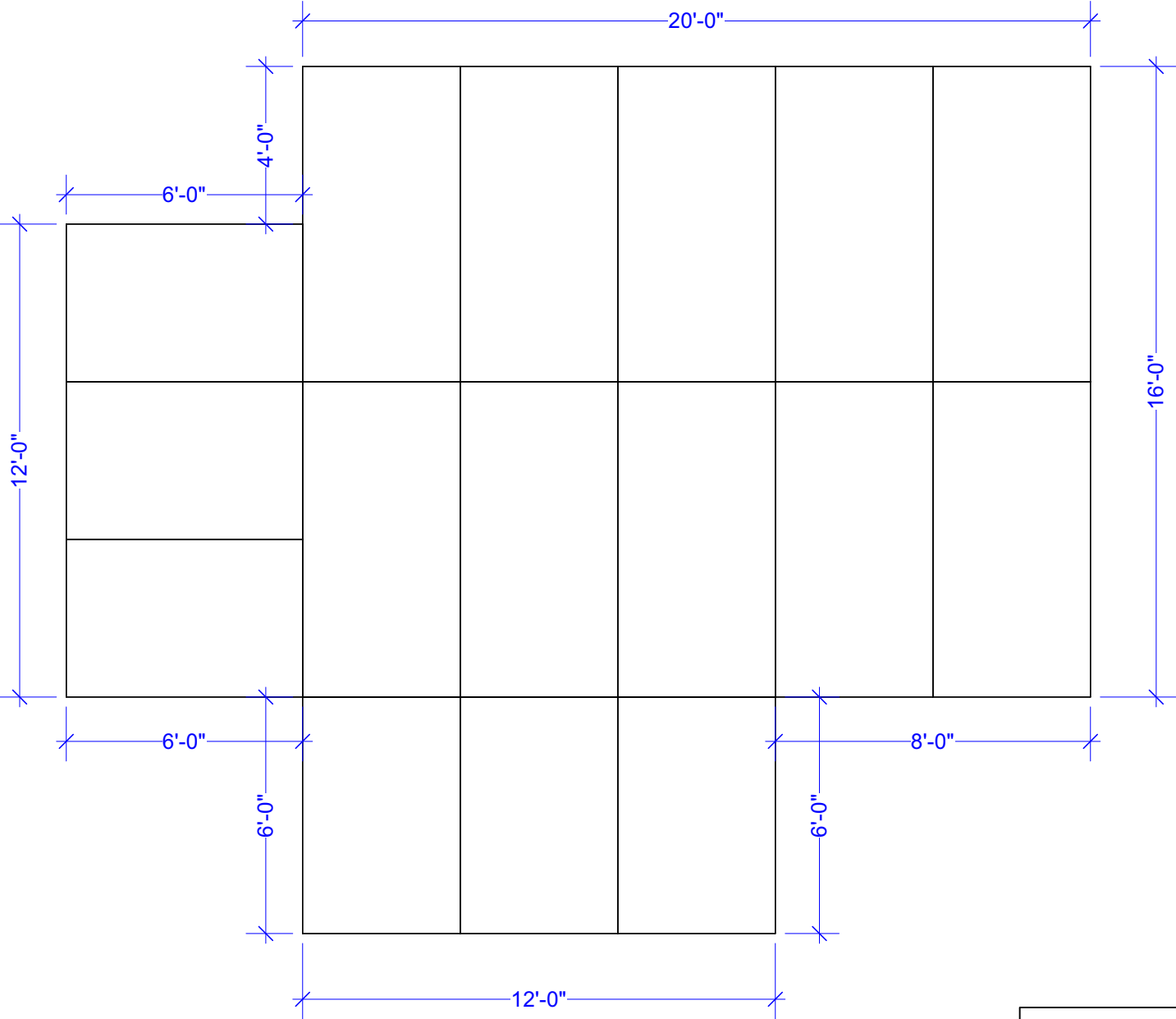
1 PLATFORMS Scale: 1/4" = 1'-0"
